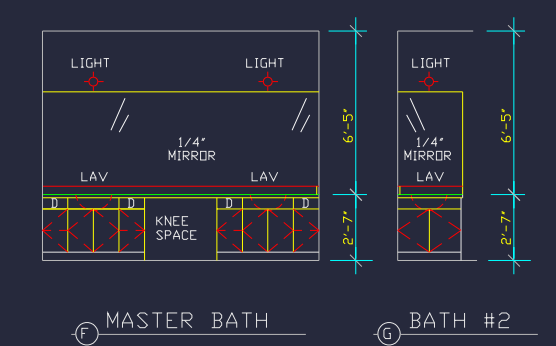
MASTER BATH
