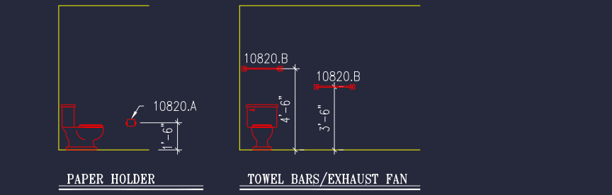
PAPER HOLDER/TOWEL BARS SCALE: 1/8" = 1'-0"
