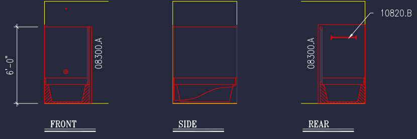
GARDEN TUB DETAILS (WITHOUT SEPARATE SHOWER) SCALE: 1/8" = 1'-0"
