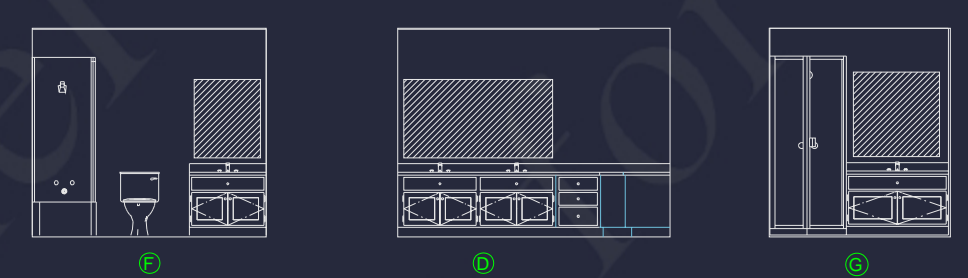
BATH ELEVATIONS SCALE: 1/4" = 1'-0"
