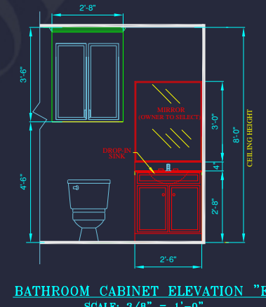
BATHROOM CABINET ELEVATION "B" SCALE: 3/8" = 1'-0"
