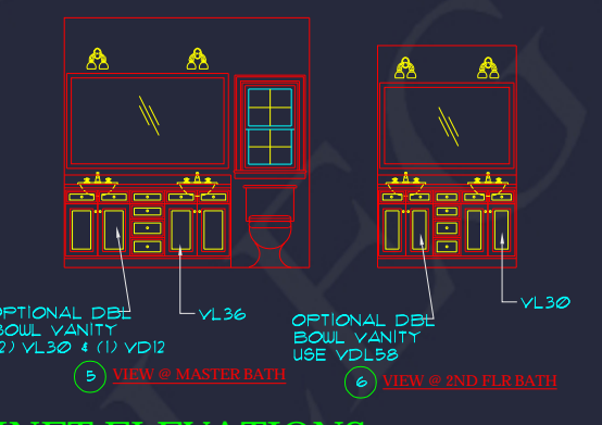
CABINET ELEVATIONS SCALE: 1/8" = 1'-0"
