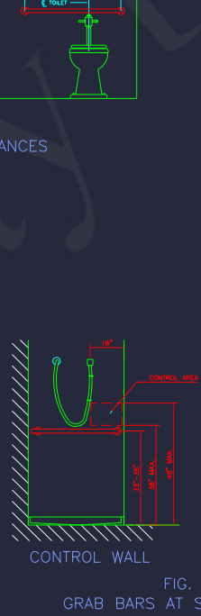
FIG. 37 GRAB BARS AT SHOWER STALLS NOTE: SHOWERHEAD AND CONTROL AREA MAY BE ON BACK (LONG) WALL (AS SHOWN) OR ON EITHER SIDE WALL
