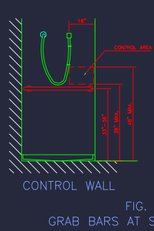
FIG. 37 GRAB BARS AT SHOWER STALLS NOTE: SHOWERHEAD AND CONTROL AREA MAY BE ON BACK (LONG) WALL (AS SHOWN) OR ON EITHER SIDE WALL
