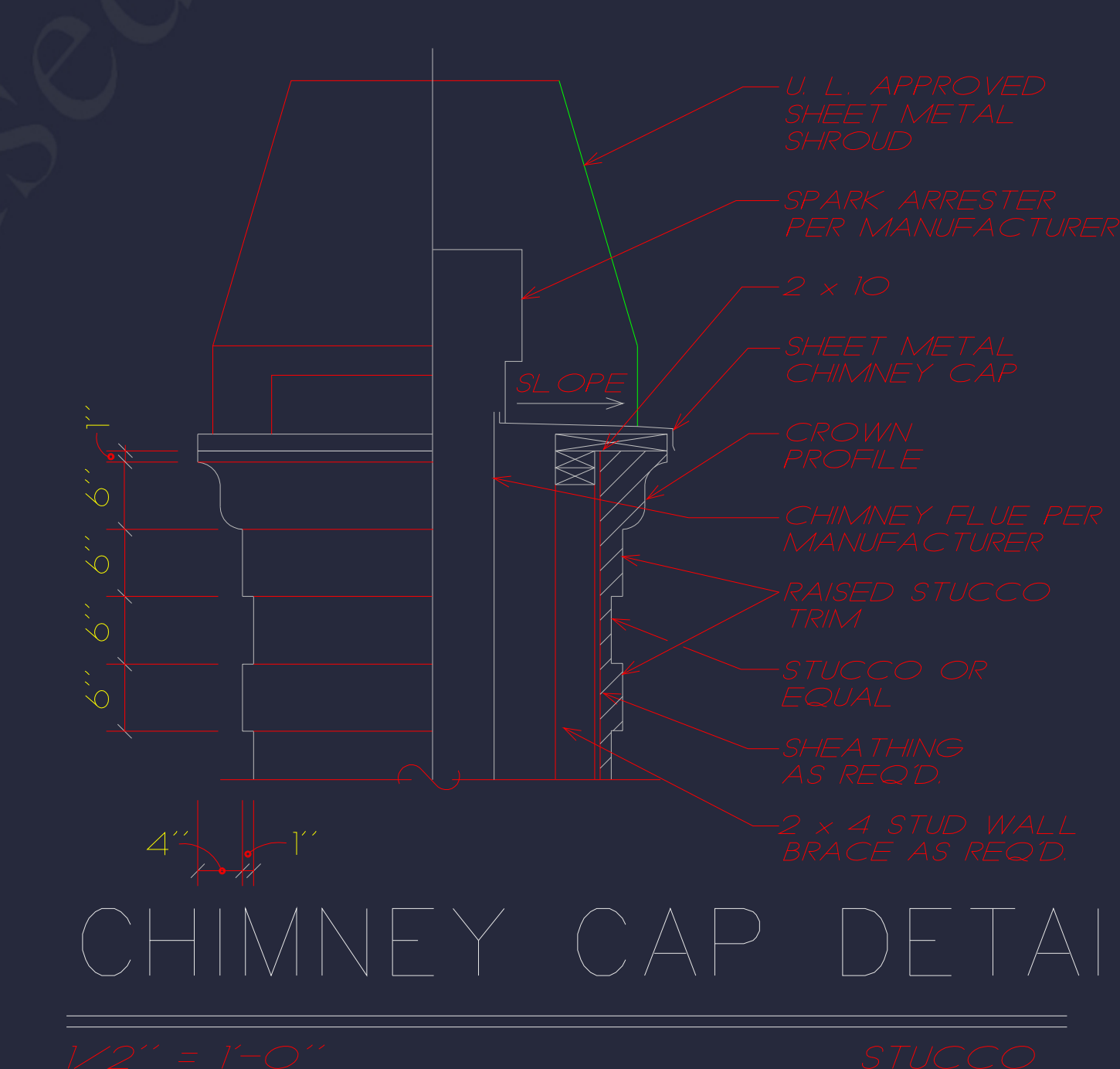
CHIMNEY CAP DETAIL
